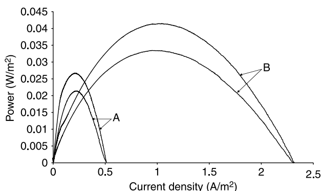
Figure 2 | Polarization curves for a non-catalyzed (A) and biocatalyzed (B) carbon tape cathode in an open air configuration. A polarization curve expresses the attainable power in function of the current flowing through a system, in this case the microbial fuel cell. A maximal power of 42 mW per m 2 cathode surface could be obtained in this case.
