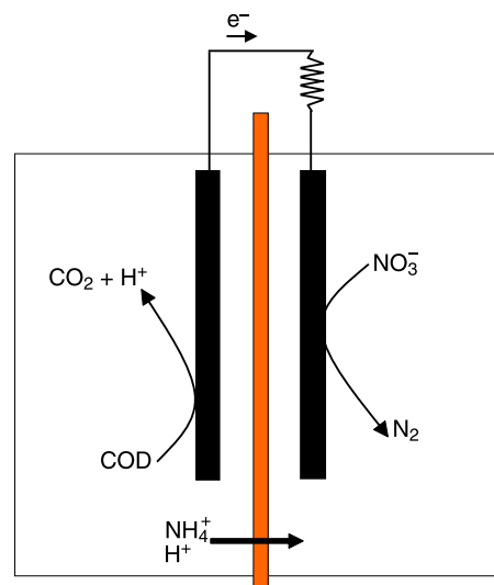
Figure 3 | Schematic representation of cathodic denitrification, driven by the anodic oxidation of acetate. The anodic process delivers electrons at a potential which is low enough to harvest power at the external resistor and still allow for the cathodic process. This implies that denitrifying bacteria can use an insoluble electron donor with a potential of around 0 mV.
