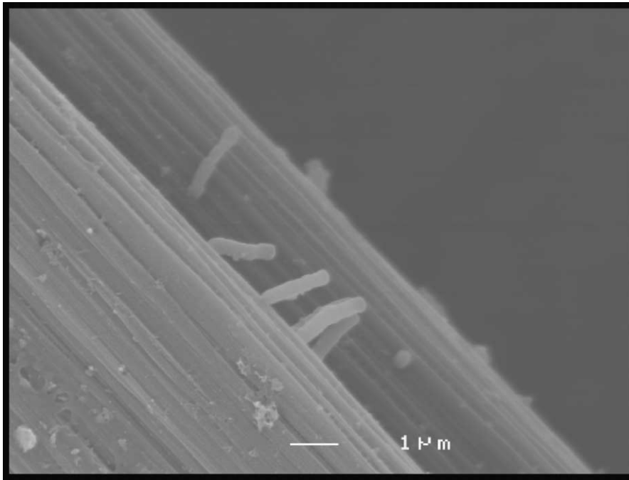
Figure 4 | Scanning electron microscopy image of a carbon fibre on which bacteria attach perpendicularly. This demonstrates that the carbon fibre surface is too smooth for bacteria to adhere to. Functionalizing the surface or selecting alternative carbon based structures may alleviate this.
