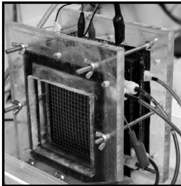
Figure 1 | Open air, biocatalyzed microbial fuel cells. The cathode comprises of a 1 mm thick carbon tape layer, covered by a stainless steel current collector. Effluent originating from the anode is recirculated over this cathode, which provides a polishing of the effluent and carry over of protons. Bacteria growing on the cathode function as biocatalyst when taking up the electrons originating from the cathode and using them to reduce oxygen.
