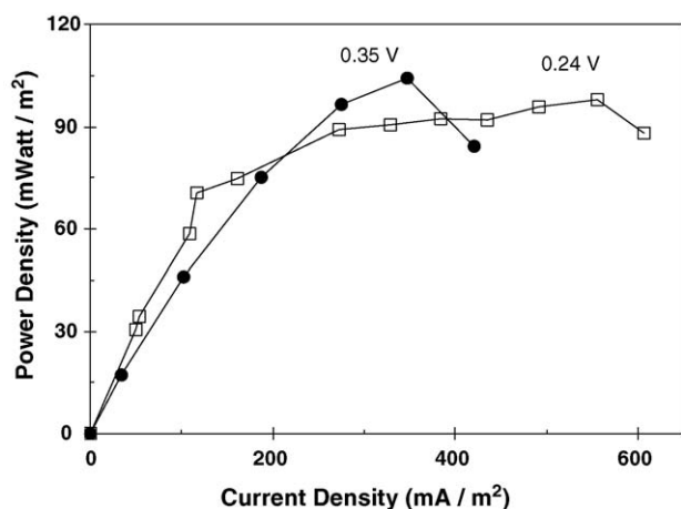
Fig. 4. Power density vs. current density curves for a fuel cell operated in Tucker-ton, NJ utilizing first an AQDS-modified anode (□) and then a graphite ceramic anode containing Mn 2+ and Ni 2+ (●). Voltage at maximum achieved power indicated.
