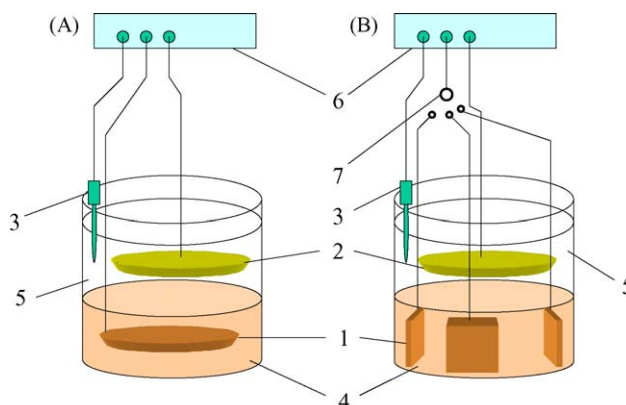
Fig. 2. Schematic of the microbial fuel cells used for recording OCP and Tafel plots: (A) system equipped with disk electrodes, (B) system equipped with three anodes. (1), Anode buried in sediment; (2), Cathode immersed in sea water; (3), Ag/AgCl, sat. KCl reference; (4), Marine sediment; (5), 2 L glass beaker; (6), Electrochemical workstation; (7), Switch for connecting various chemically modified anodes.
