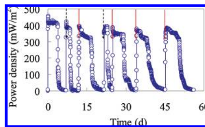
FIGURE 3. Power densities of MFC CSRS using corn stover residual solids after steam explosion.
