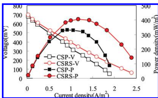
FIGURE 2. Power output and power density curve of MFCs using raw corn stover powder (CSP; MFC CSP ) and corn stover residual solids after steam explosion (CSRS; MFC CSRS ) as substrate.
