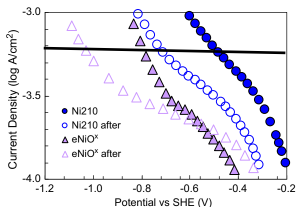
Fig. 4 – Examples of Tafel plots for cathodes before and after use in 12 MEC cycles. Test conditions: 2 mM phosphate buffer, scan rate 2 mV/s, third scan.
