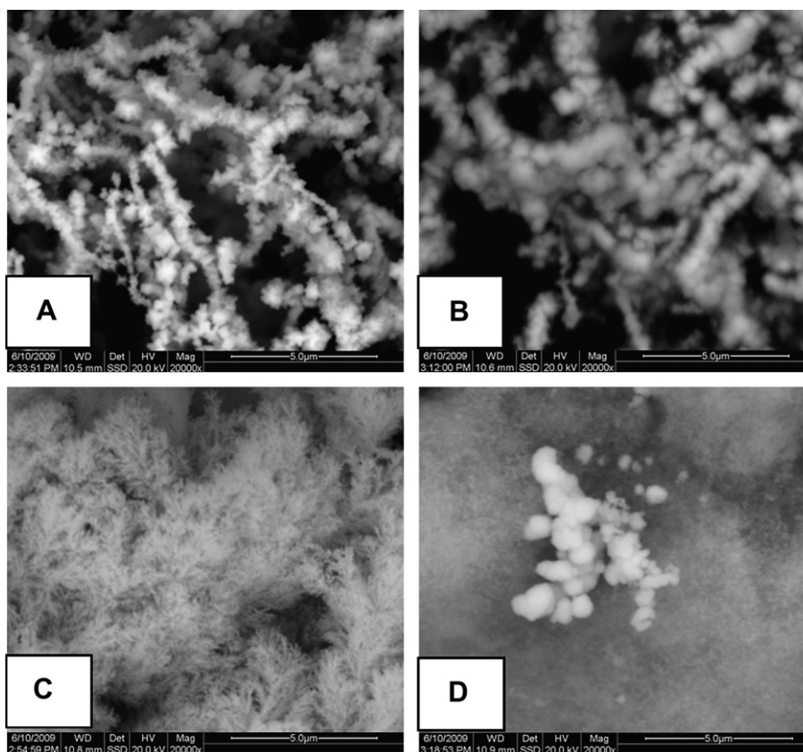
Fig. 5 – SEM images of Ni 210 catalyst cathodes (A and B) and eNiOx catalyst cathodes (C and D), before (A and C) and after (B and D) 12 cycles in MEC. Images are at 20,000 × magnification.
