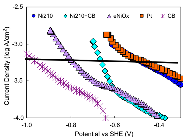
Fig. 1 – Tafel plots for select experimental cathodes in 2 mM phosphate buffer, scan rate 2 mV/s, third scan.
