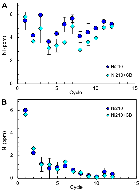
Fig. 6 – Nickel content via ICP-AES analysis in MEC solution after (A) aerobic feeding and (B) anaerobic feeding.
