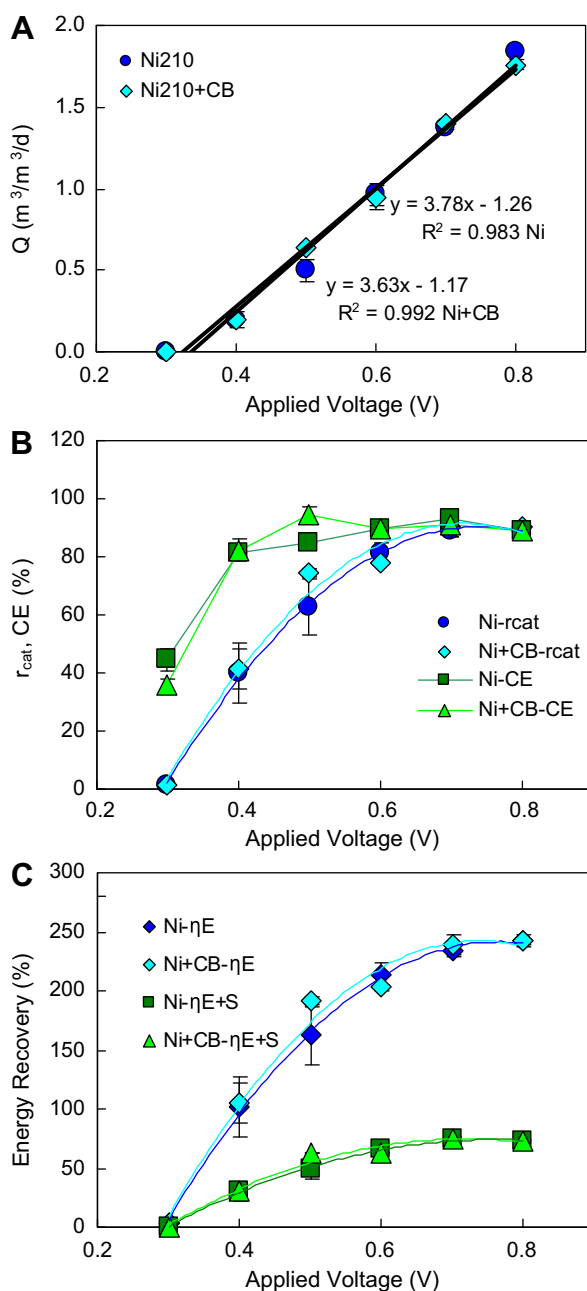
Fig. 3 – MEC performance for Ni 210 catalyst cathodes at different applied voltages. (A) hydrogen production rate (B) cathodic recovery and coulombic efficiency (C) energy recovery based on electrical input and overall energy recovery.
