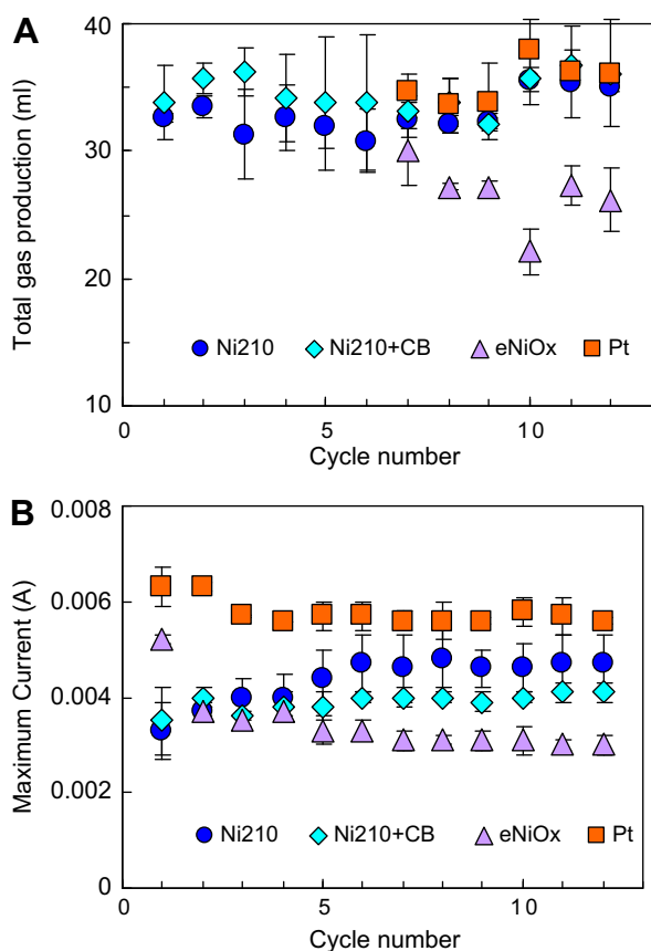
Fig. 2 – (A) Total gas production and (B) maximum current for MECs with Ni 210, Ni 210 + CB, eNiO x or Pt catalyst cathodes, as a function of cycle number at an applied voltage of 0.6 V. Gas production for cycles 1–6 were not recorded for Pt and eNiO x due to equipment malfunction.
