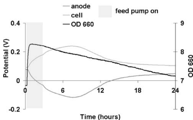
Fig. 4 Typical daily characteristics of the MFC of PAMFC 1 showing the anode potential, cell voltage, and the optical density of the algae suspension calculated from the online turbidity measurements during day 125. The applied external resistance was 25 \Omega . The gray area represents the feeding period
