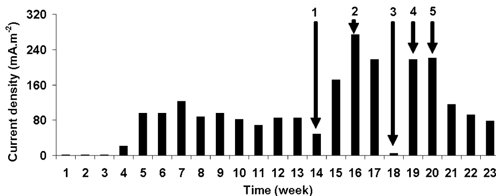
Fig. 2 Long-term operation of the PAMFCs showing the average week current density per square meter projected anode surface. 1 Installment of AR2; this photobioreactor had a higher algae productivity since the maximum OD660 of AR2 was 1.3 times higher than AR1. In week 14, this did not result in a higher current density, since algae productivity was lost due a leakage. In week 15, the current density was 171 \text{ mA m}^{-2} , so the installment of AR2 resulted in a more current generation compared to AR1. 2 External resistance was
